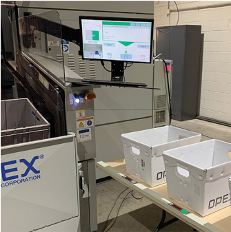
Pick-to-table
